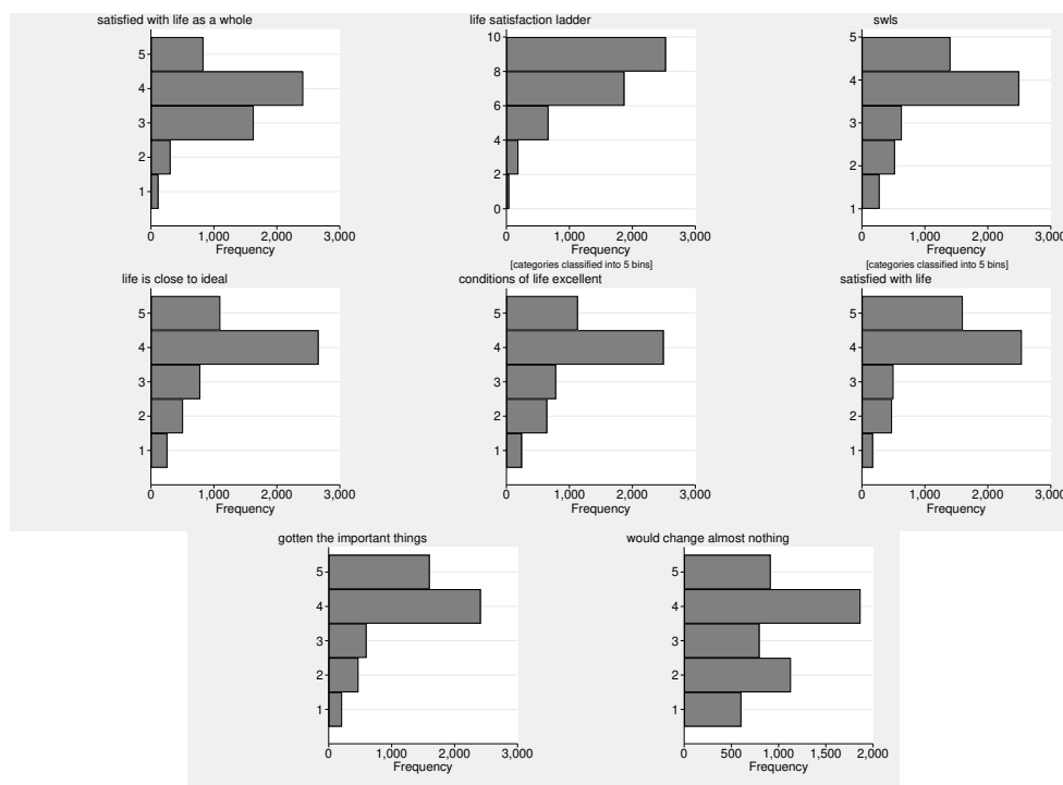
Figure 2: Variables' distribution.
